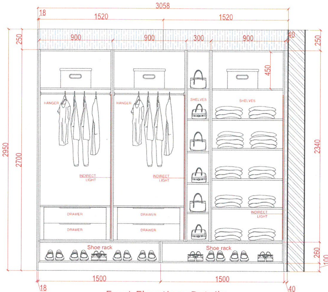
Front Elevations Details
