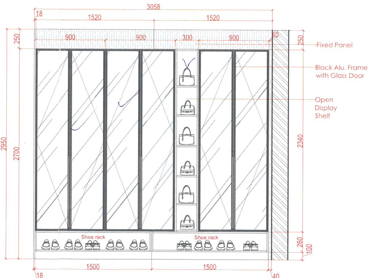
Front Elevations Details with Doors
